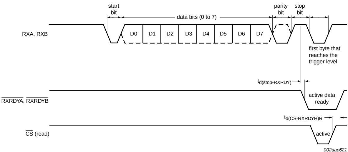
Fig 23. Receive ready timing in FIFO mode (68 mode)
