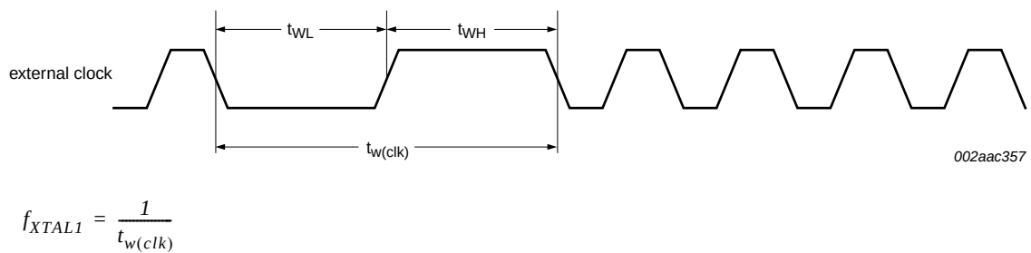
Fig 15. External clock timing
