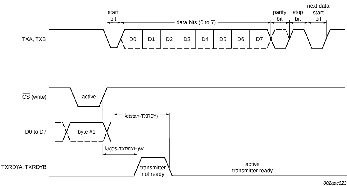
Fig 27. Transmit ready timing in non-FIFO mode (68 mode)
