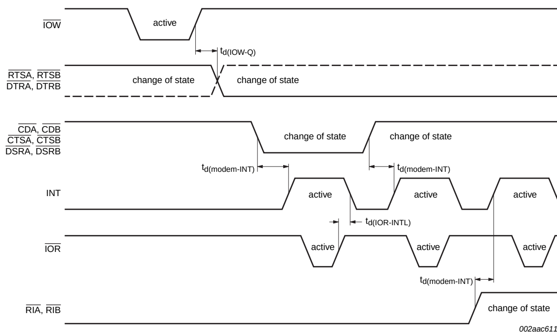
Fig 16. Modem input/output timing in 16 mode
