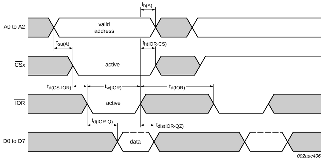
Fig 13. General read timing in 16 mode
