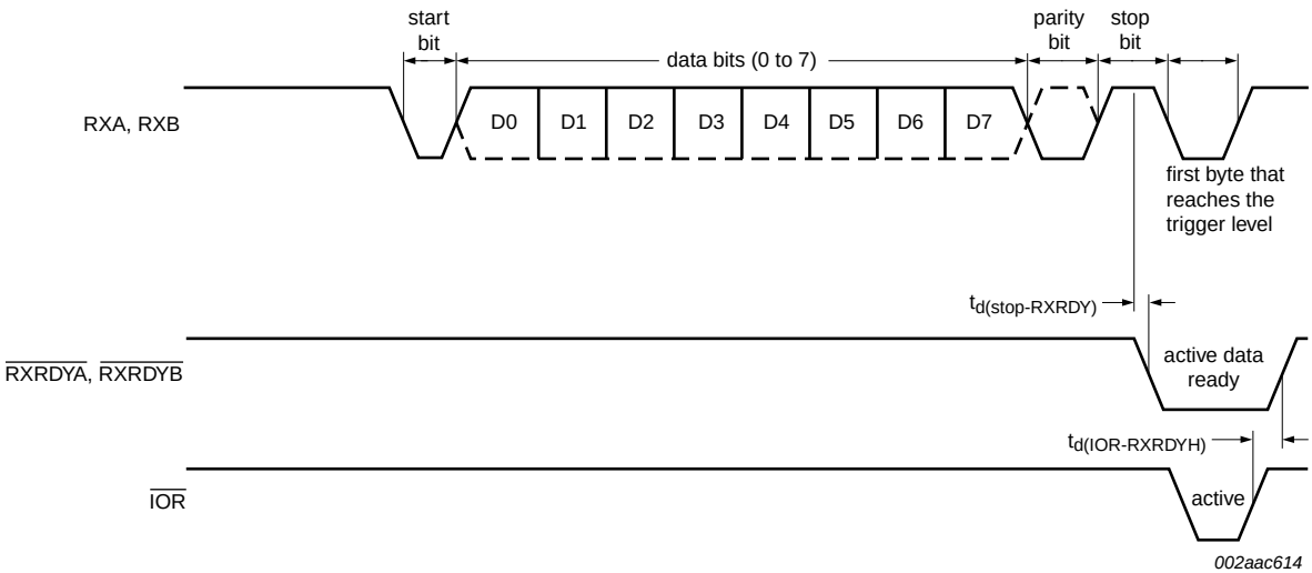
Fig 22. Receive ready timing in FIFO mode (16 mode)
