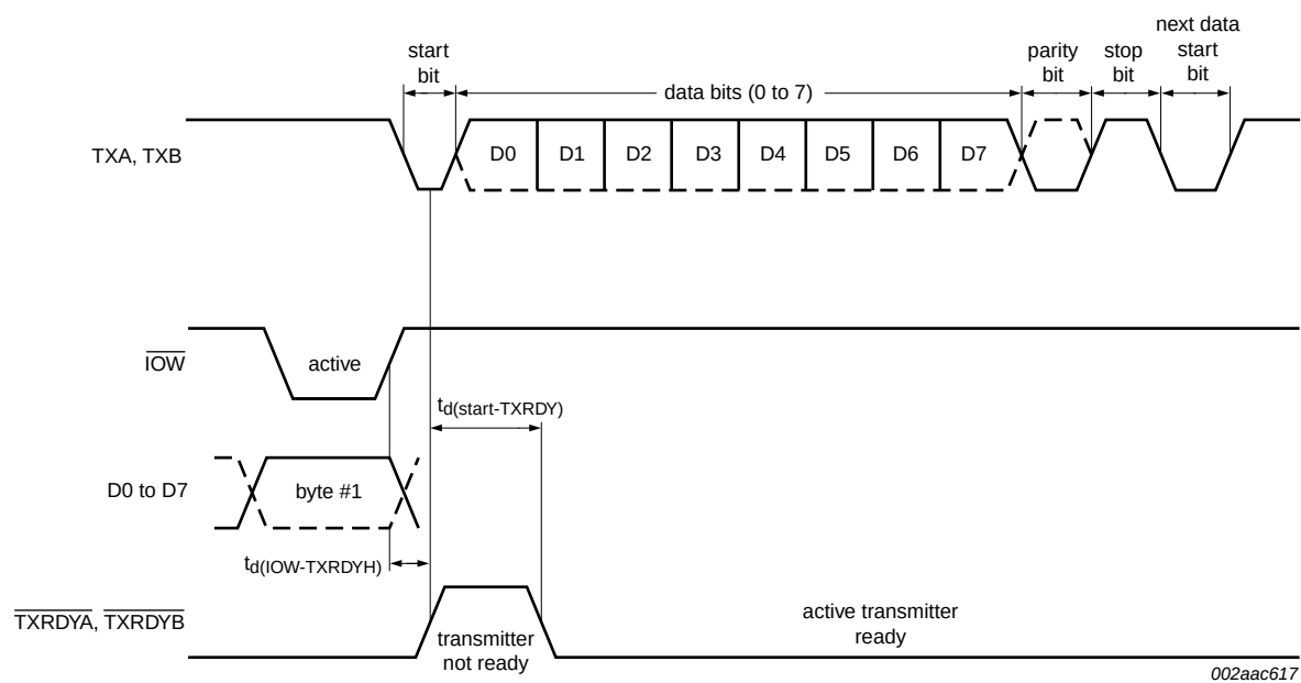
Fig 26. Transmit ready timing in non-FIFO mode (16 mode)
