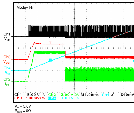
Start Up (Enable) into Output Short Circuit
