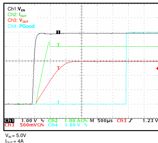
Start Up (Enable) ( V_{OUT} = 1.5V ) @ Full Load
