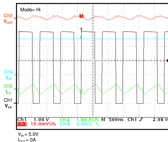
Output Voltage Ripple ( V_{OUT} = 3.3V ), forced PWM
