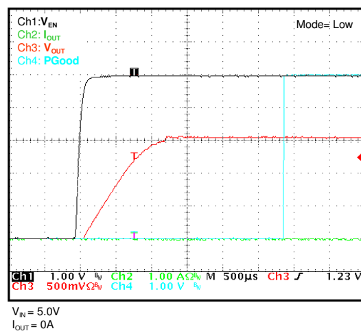
Start Up (Enable) ( V_{OUT} = 1.5V ), PSAVE Mode
