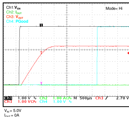
Start Up (Enable) ( V_{OUT}=3.3V ), forced PWM
