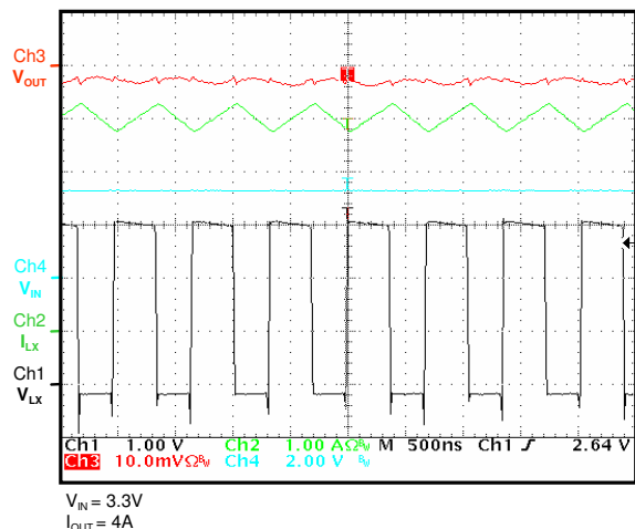
Output Voltage Ripple ( V_{OUT}=1.5\text{V} ) @ Full Load
