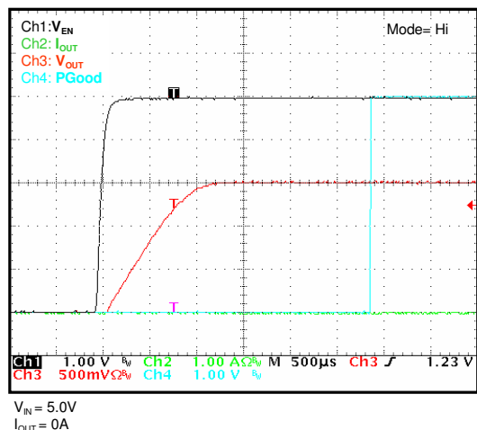
Start Up (Enable) ( V_{OUT} = 1.5V ), forced PWM
