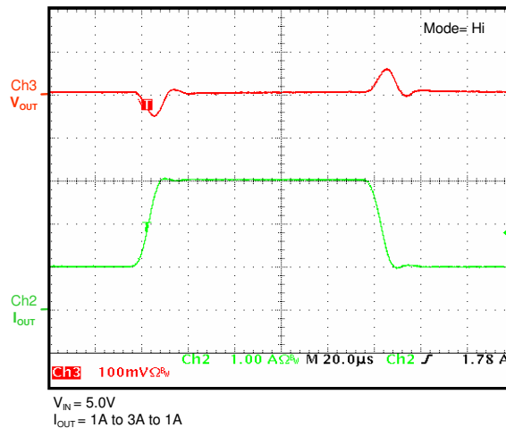
Transient Response ( V_{OUT}=3.3V , I_{STEP}=2A )
