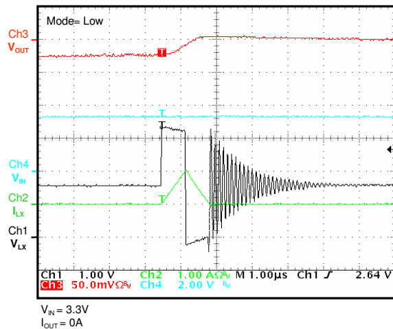
Output Voltage Ripple ( V_{OUT}=1.5V ), PSAVE Mode
