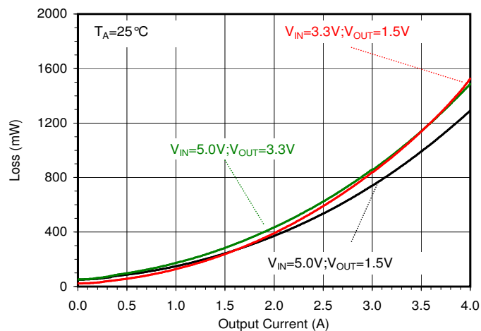
Total Loss (Forced PWM)
