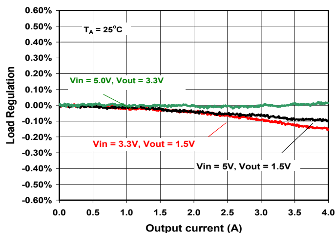
Load Regulation (Forced PWM)
