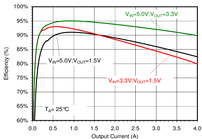
Efficiency (Forced PWM)
