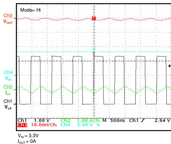
Output Voltage Ripple ( V_{OUT}=1.5V ), Forced PWM
