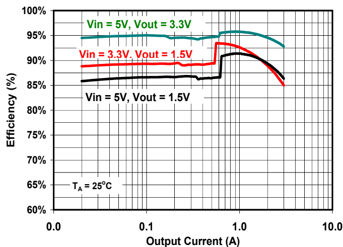
Efficiency (PSAVE Enabled)
