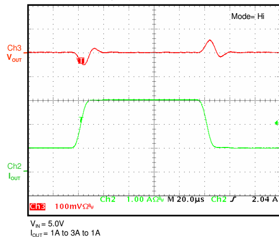
Transient Response ( V_{OUT}=1.5V , I_{STEP}=2A )
