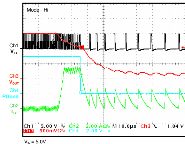
Output Short Circuit ( V_{OUT}=1.5V )
