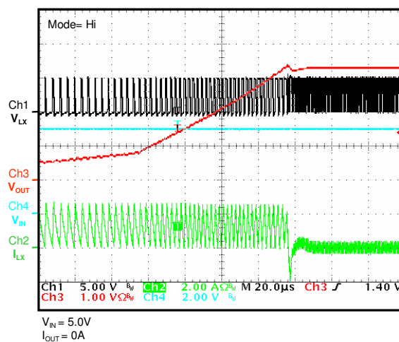
Recovery from OCP ( V_{OUT}=3.3V )
