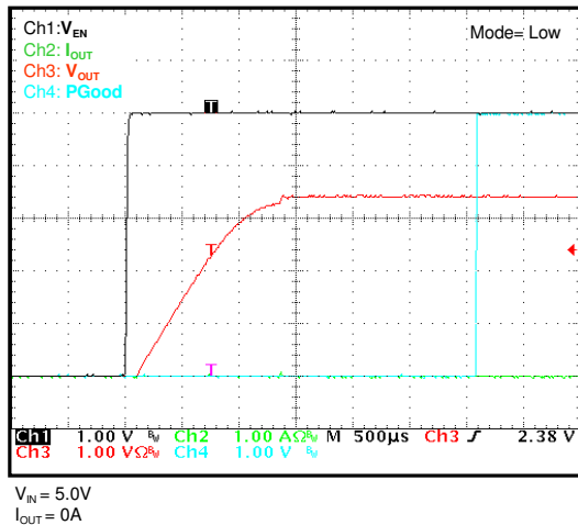
Start Up (Enable) ( V_{OUT}=3.3V ), PSAVE Mode
