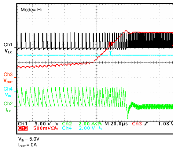
Recovery from OCP ( V_{OUT}=1.5V )
