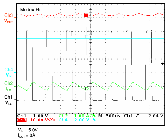
Output Voltage Ripple ( V_{OUT}=1.5V ), Forced PWM
