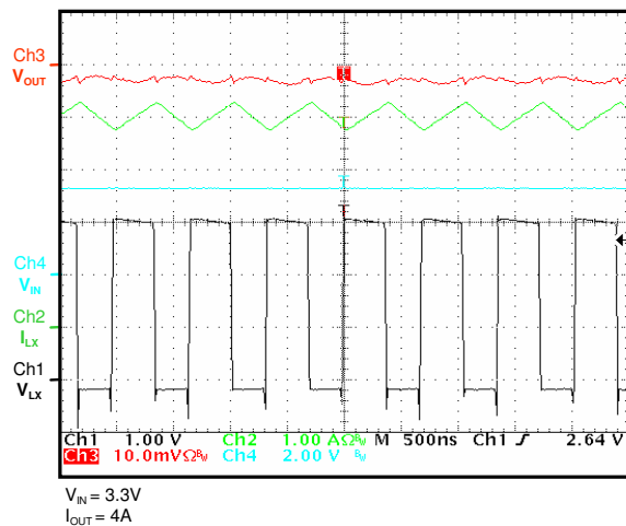
Output Voltage Ripple ( V_{OUT}=1.5V ) @ Full Load
