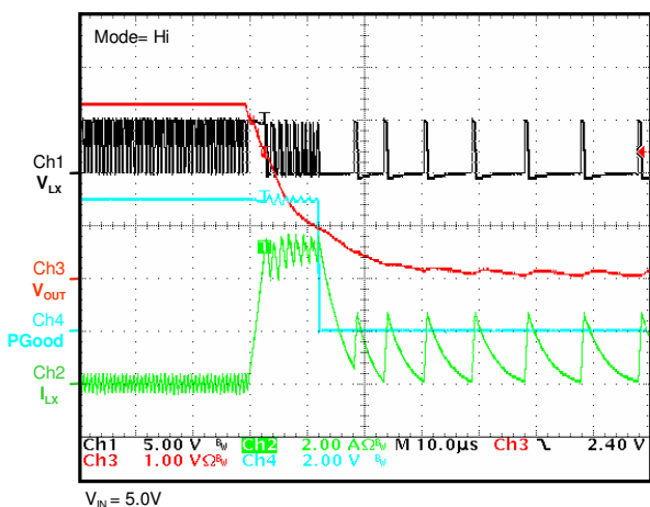
Output Short Circuit ( V_{OUT}=3.3V )
