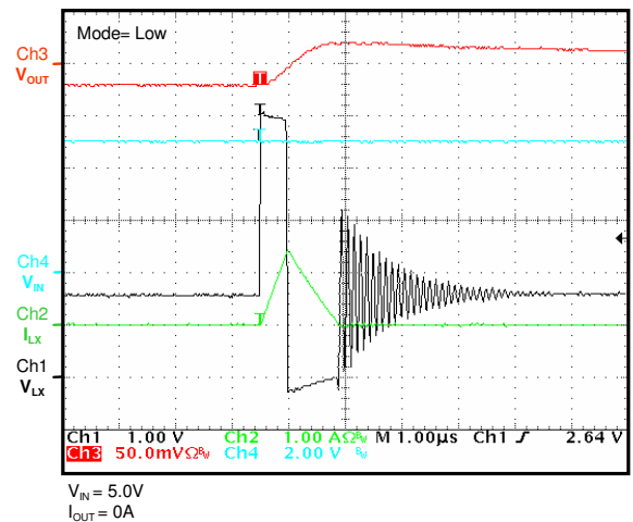
Output Voltage Ripple ( V_{OUT}=1.5V ), PSAVE Mode
