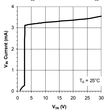
V_{IN} Quiescent Current vs V_{IN}
