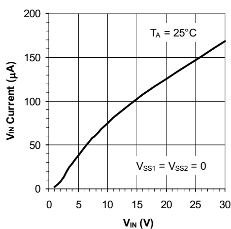
V_{IN} Shutdown Current vs V_{IN}
