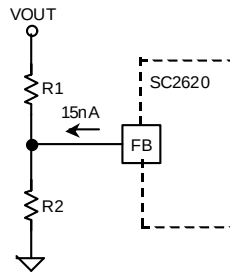
Figure 4. V_{OUT} is set with a Resistive Divider
