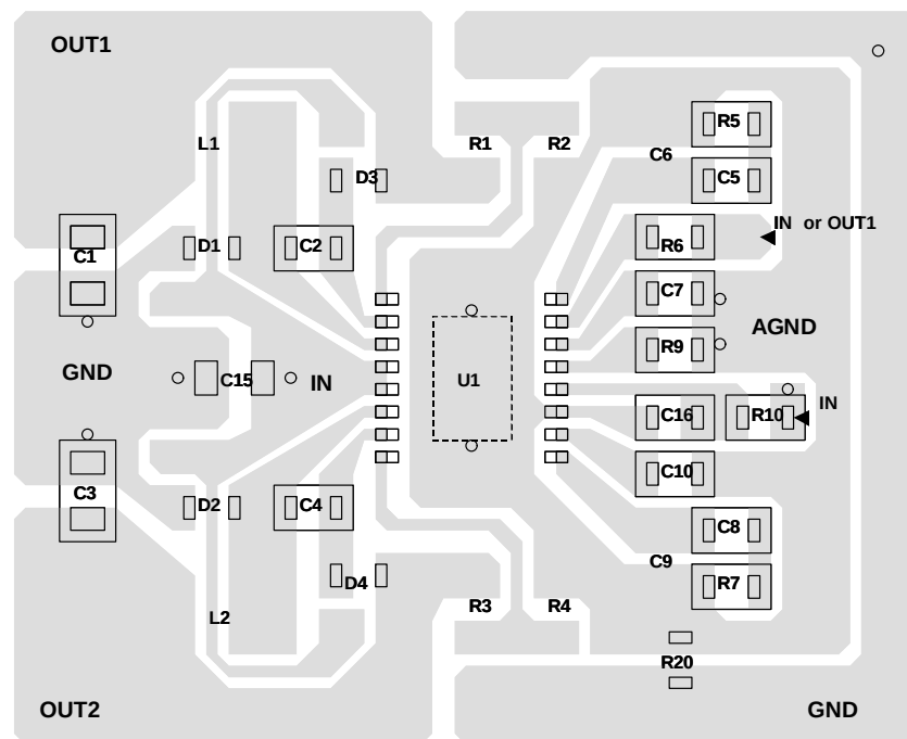
Figure 15. Suggested PCB Layout for the SC2620.
