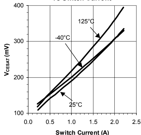
Switch Saturation Voltage vs Switch Current
