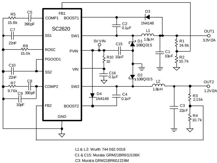
Figure 16(a). 1.2MHz 5V to 3.3V and 1.2V xDSL Power Supply. Channel 2 does not start until Channel 1 output voltage becomes regulated.
