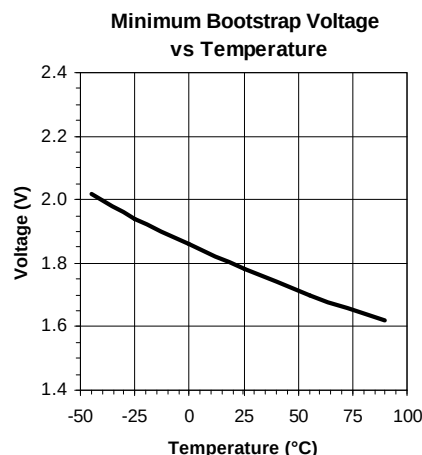
Figure 6. Typical Minimum Bootstrap Voltage Required to Maintain Saturation at I_{SW} = 2A .
