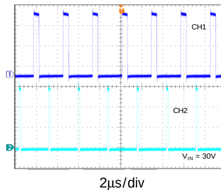
Figure 18(b). Switching Waveforms. I_{OUT1} = I_{OUT2} = 1A .
