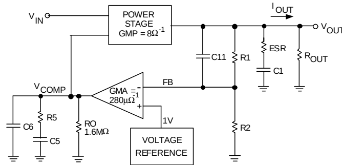
Figure 11. Simplified Control Loop Equivalent Circuit
