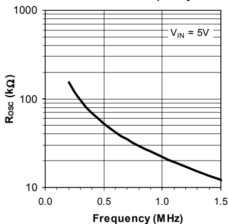
Frequency Setting Resistor vs Channel Frequency
