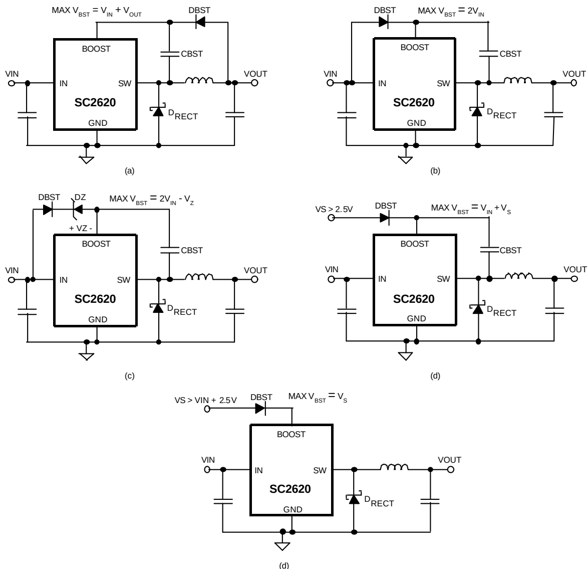
Figure 7. Methods of Bootstrapping the SC2620.
