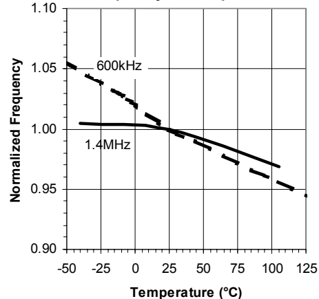
Normalized Channel Frequency vs Temperature
