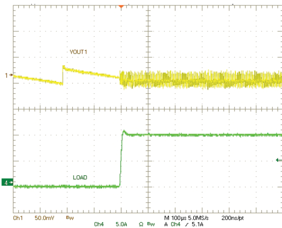
Load Step VOUT1, 1.8V
