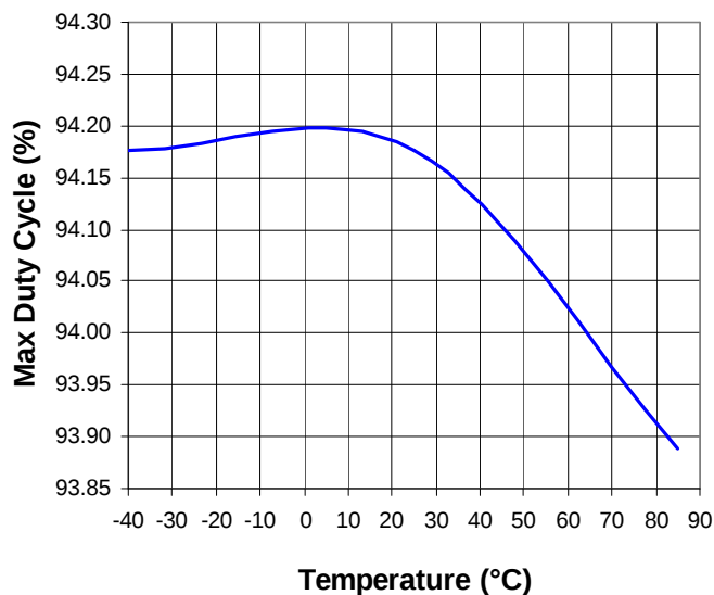
Max Duty Cycle vs Temperature @ ROSC = 220K
