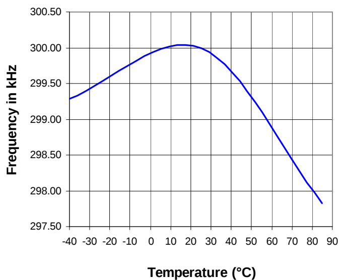
Frequency vs Temperature @ ROSC = 220K
