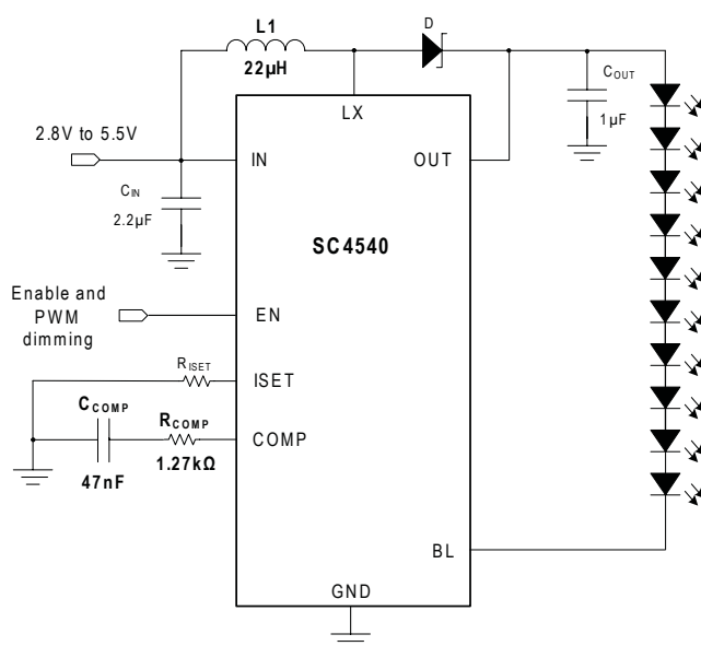
Figure 3 — Low Input Voltage Application Circuit
