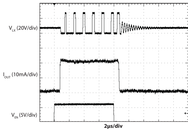
PWM Operation at 20kHz and 10% Duty Cycle
