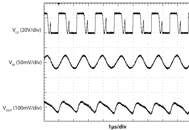
Typical Waveforms at V_{IN} = 12V
