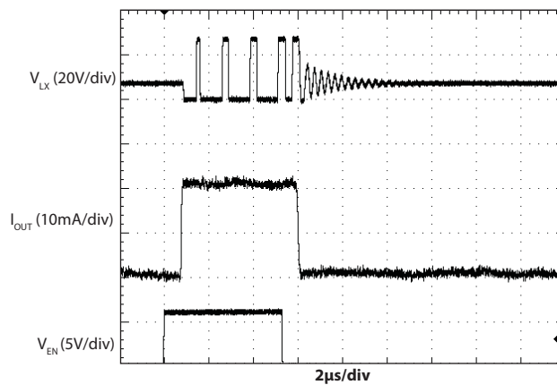
PWM Operation at 32kHz and 17% Duty Cycle
