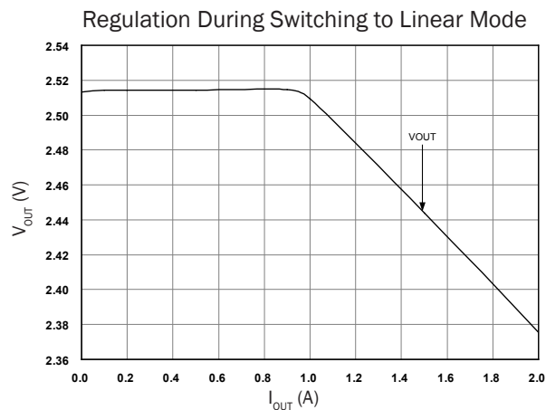
Figure 13. Loading Regulation
