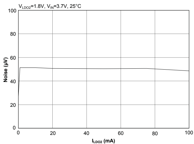
Noise vs Load Current (LDO2)
