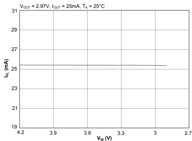
Spotlight Current — 25mA
