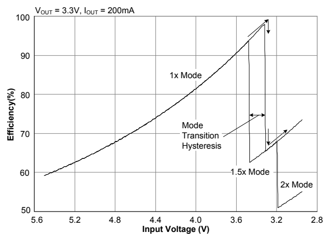
Efficiency — 200mA
