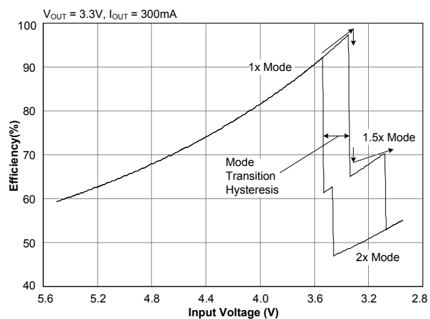
Efficiency — 300mA
