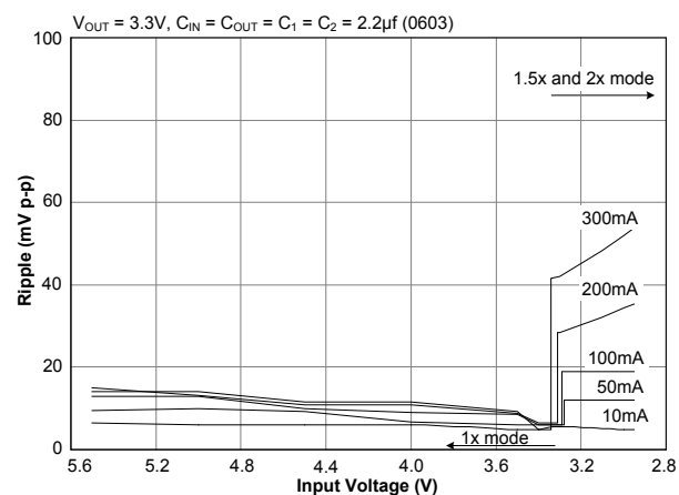
Output Ripple
