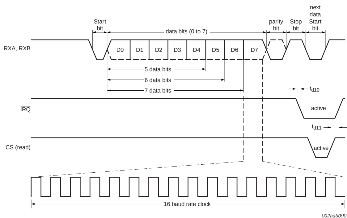
Fig 9. Receive timing
