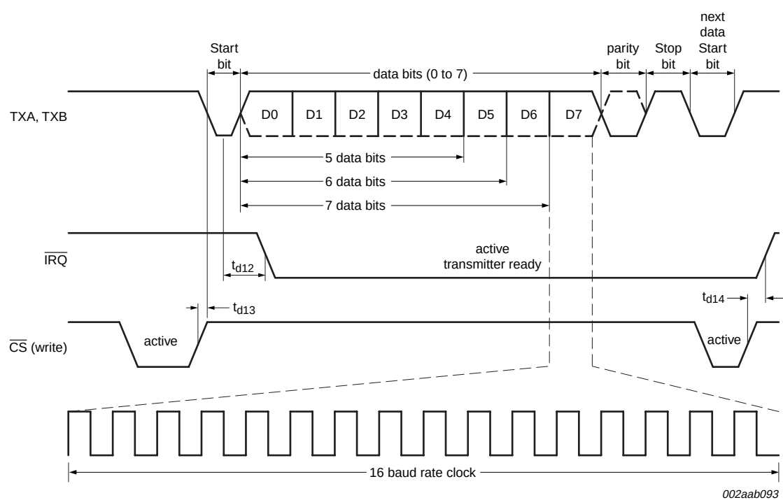
Fig 12. Transmit timing
