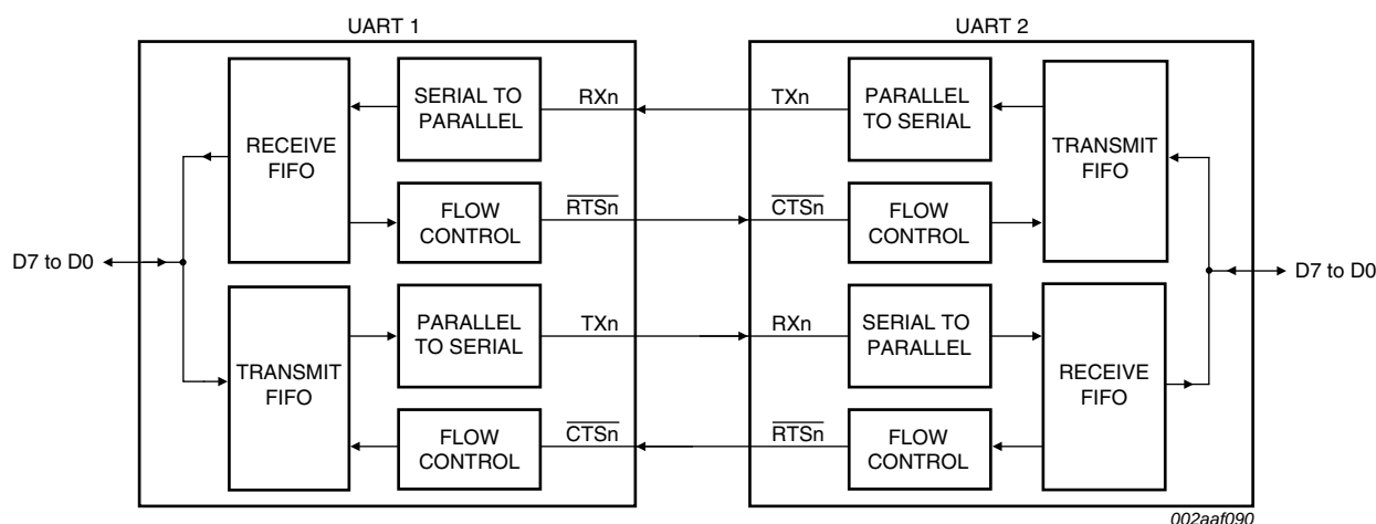
Fig 4. Auto flow control ( \overline{\text{auto-RTS}} and \overline{\text{auto-CTS}} ) example
