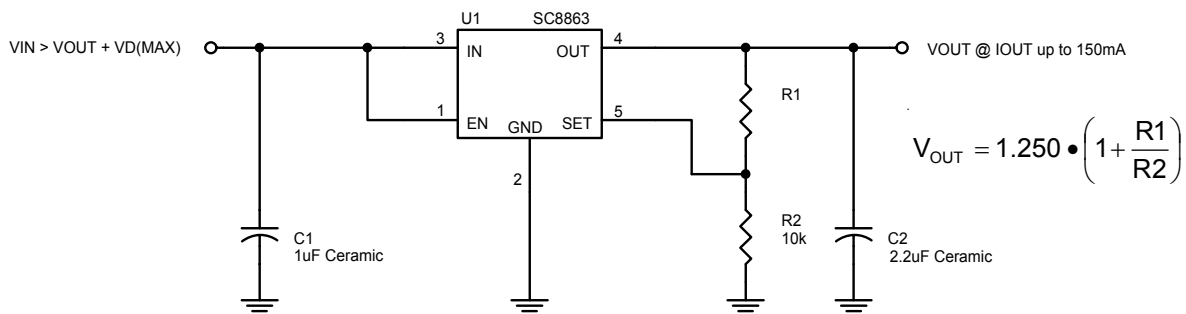
Externally Preset Output Voltage (1)
