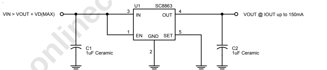
Internally Preset Output Voltage
