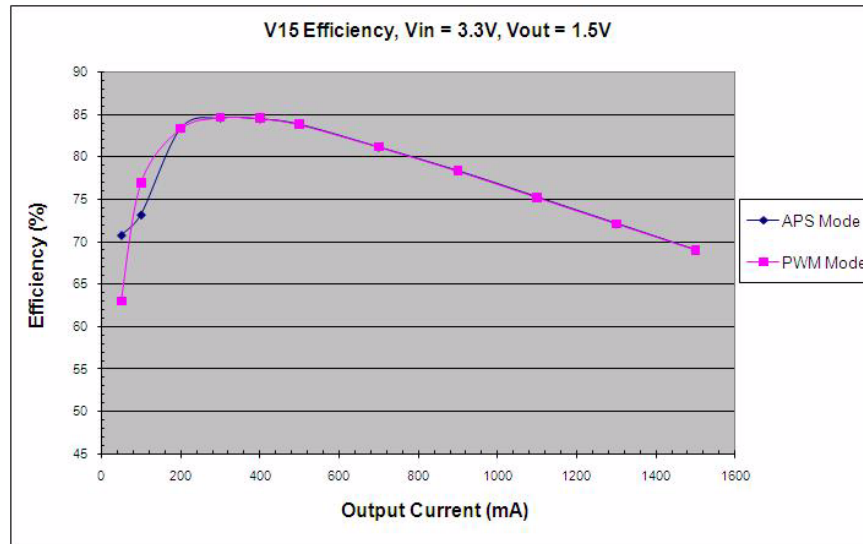
Figure 33. V15 Efficiency Curves
