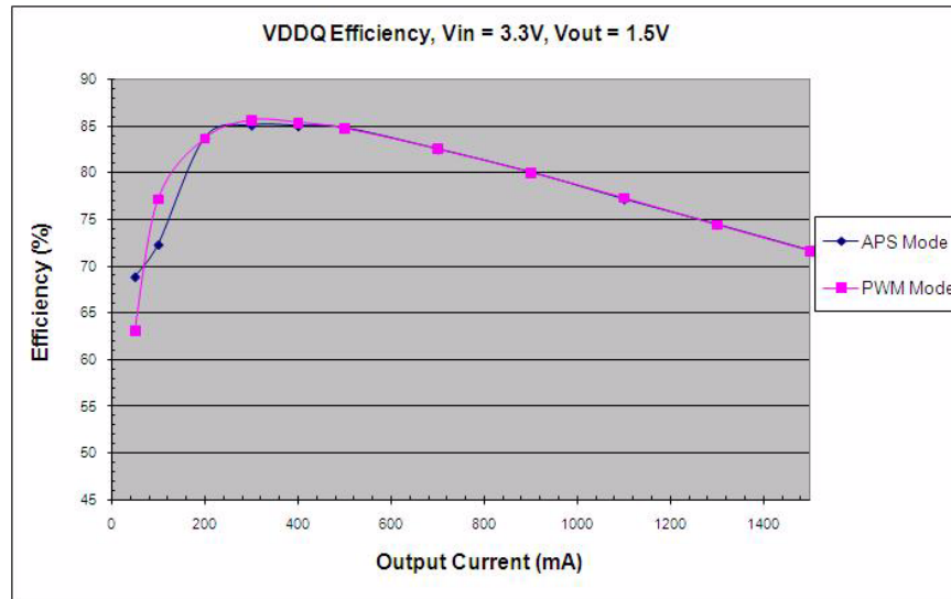
Figure 29. VDDQ Efficiency Curves
