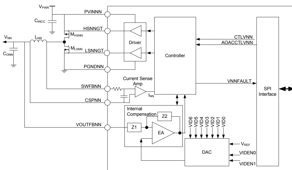
Figure 25. VNN Detailed Internal Block Diagram
