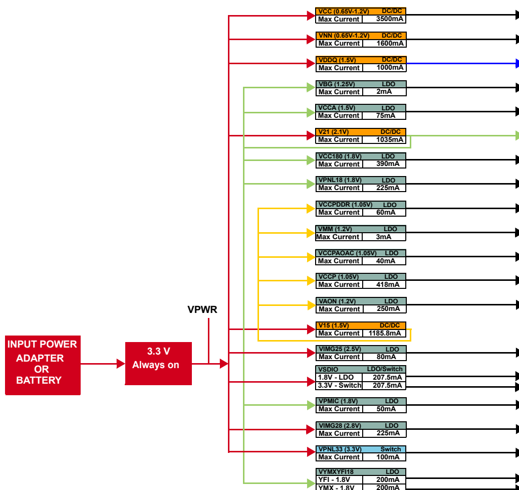
Figure 22. 900844 Power Map
