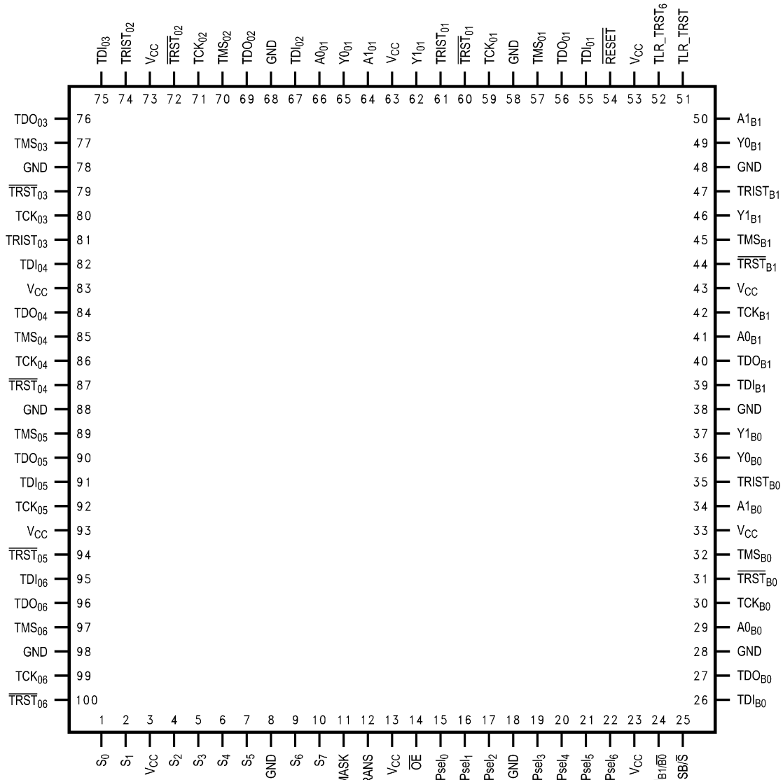
TQFP pinout
