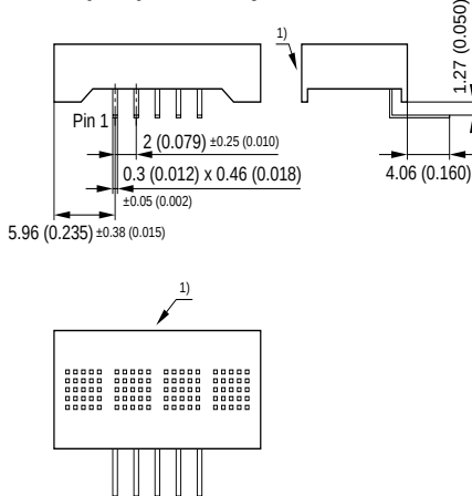
SCDQ554XQ 90° SIP Package
