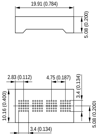
SCDQ554XQ 90° SIP Package
