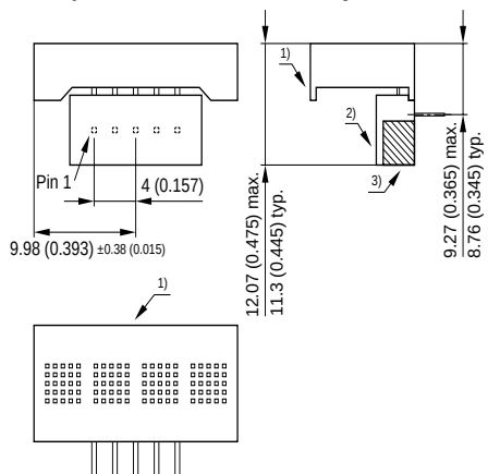
SCDQ554XR 90° Connector/Header Package
