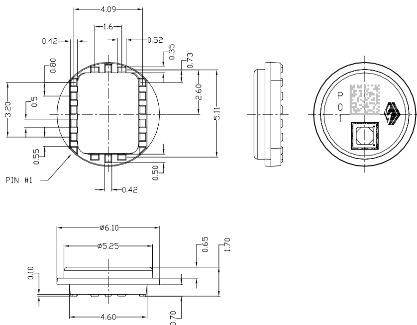
Figure 19. SCP1000 package dimensions.
