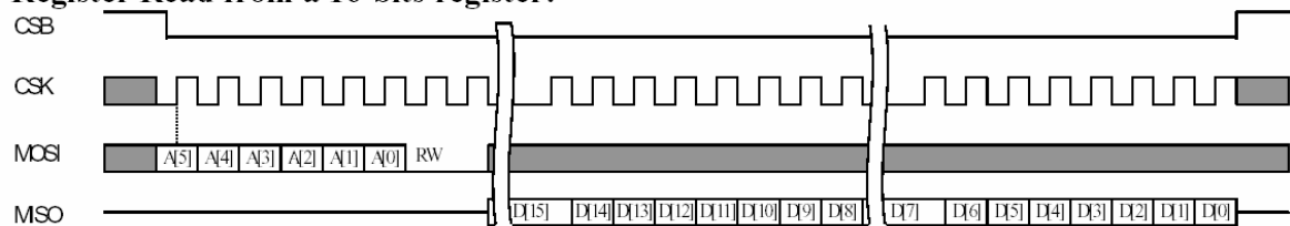
Figure 10. SPI communication examples.
