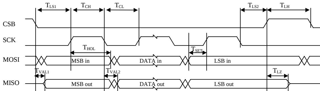
Figure 17. Timing diagram for SPI communication.
