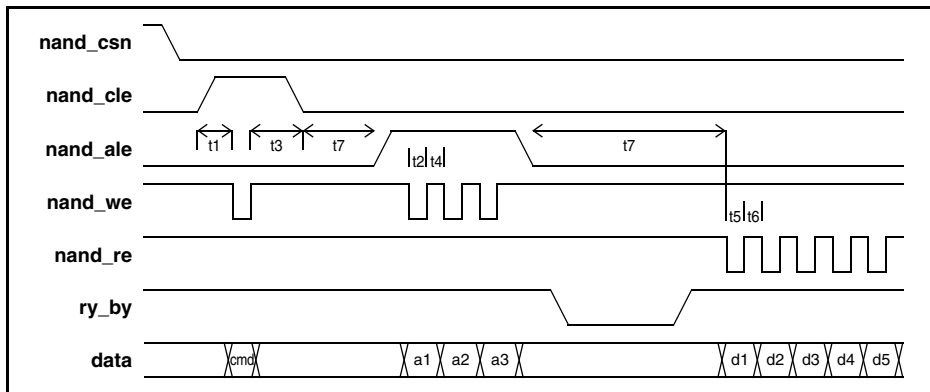
Figure 17. NAND Flash Page Read Cycle
