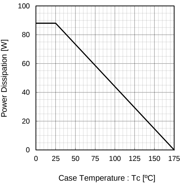
Fig.6 Power Dissipation
