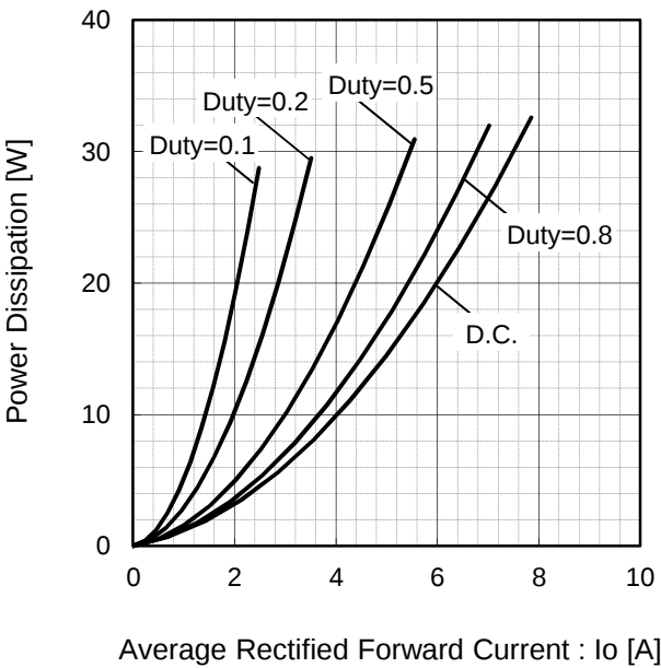
Fig.8 Io-Pf Characteristics
