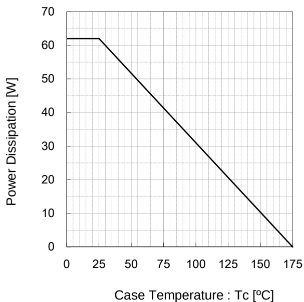
Fig.6 Power Dissipation
