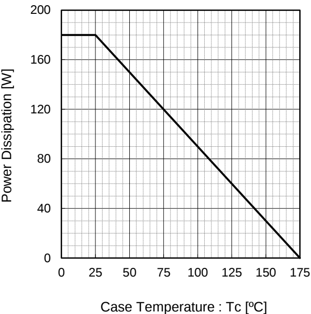
Fig.6 Power Dissipation
