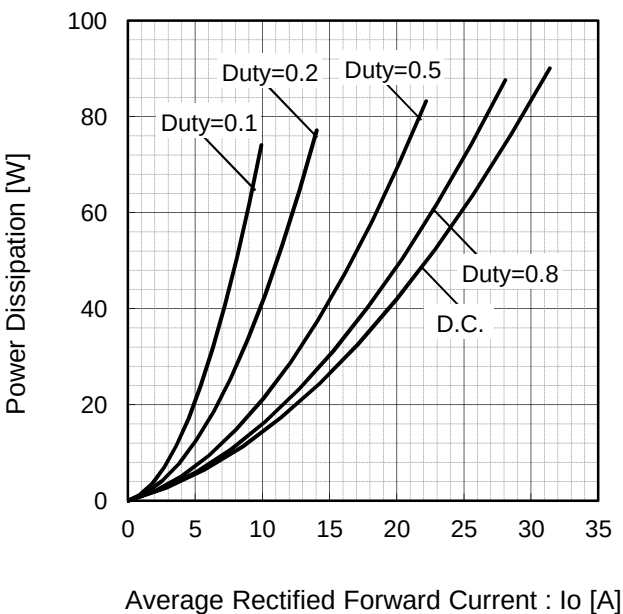
Fig.8 Io-Pf Characteristics
