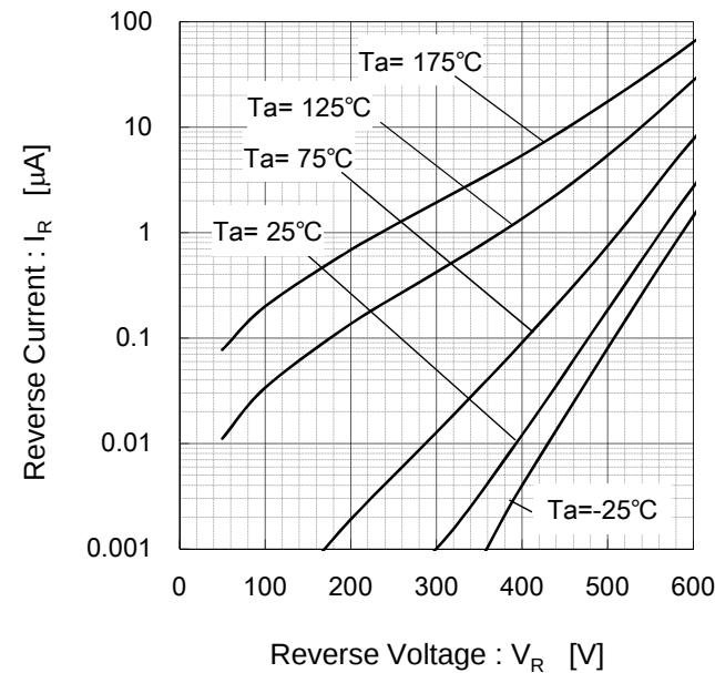
Fig.3 V_R - I_R Characteristics (Per leg)
