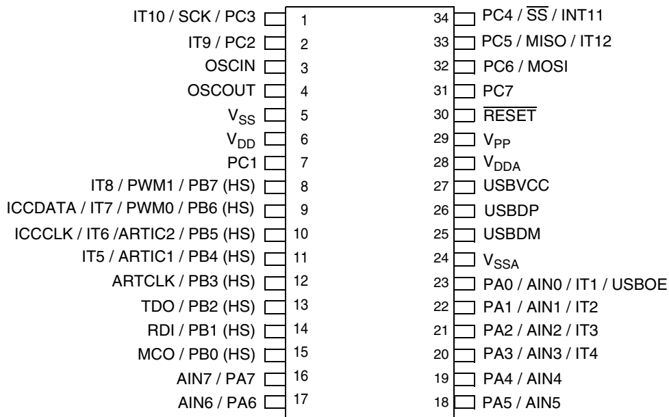
Figure 3. 34-Pin SO and 32-Pin SDIP Package Pinouts
