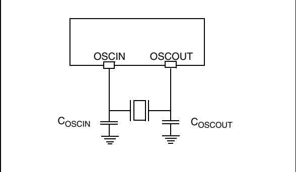
Figure 13. Crystal/Ceramic Resonator
