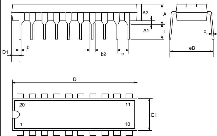
Figure 91. 20-Pin Plastic Dual In-Line Package, 300-mil Width
