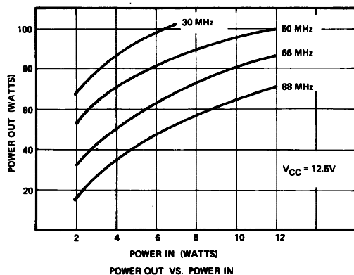
Figure 3. Power Output vs Power Input
