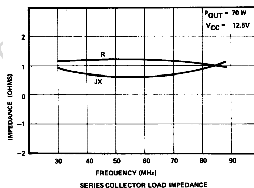
Figure 5. Typical Collector Load Impedance
