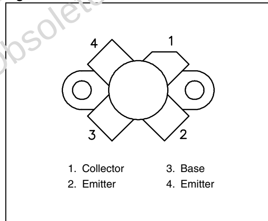
Figure 2. Pin Connection
