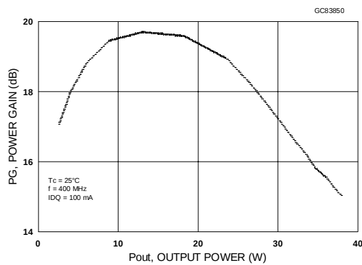
Power Gain vs Output Power
