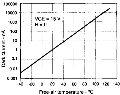
Fig. 3 Dark Current vs Temperature gra_303.cdr
