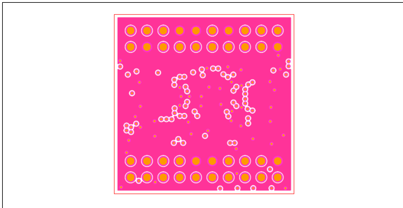
Figure 5-4. Wiring layout (layer 2)
