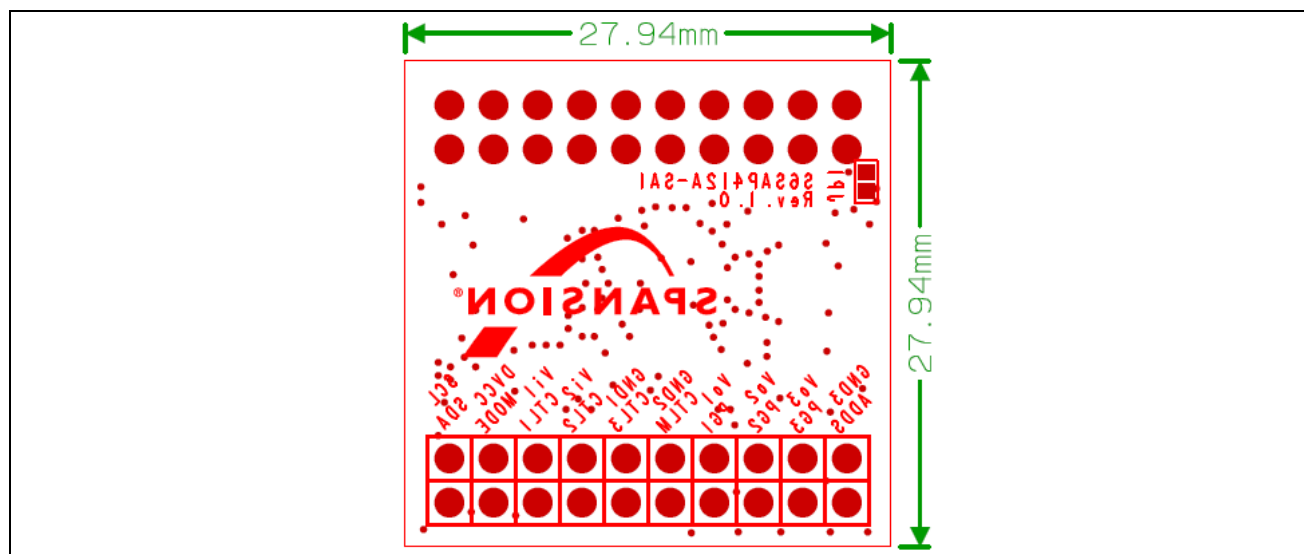
Figure 5-2. Component layout (layer 4)
