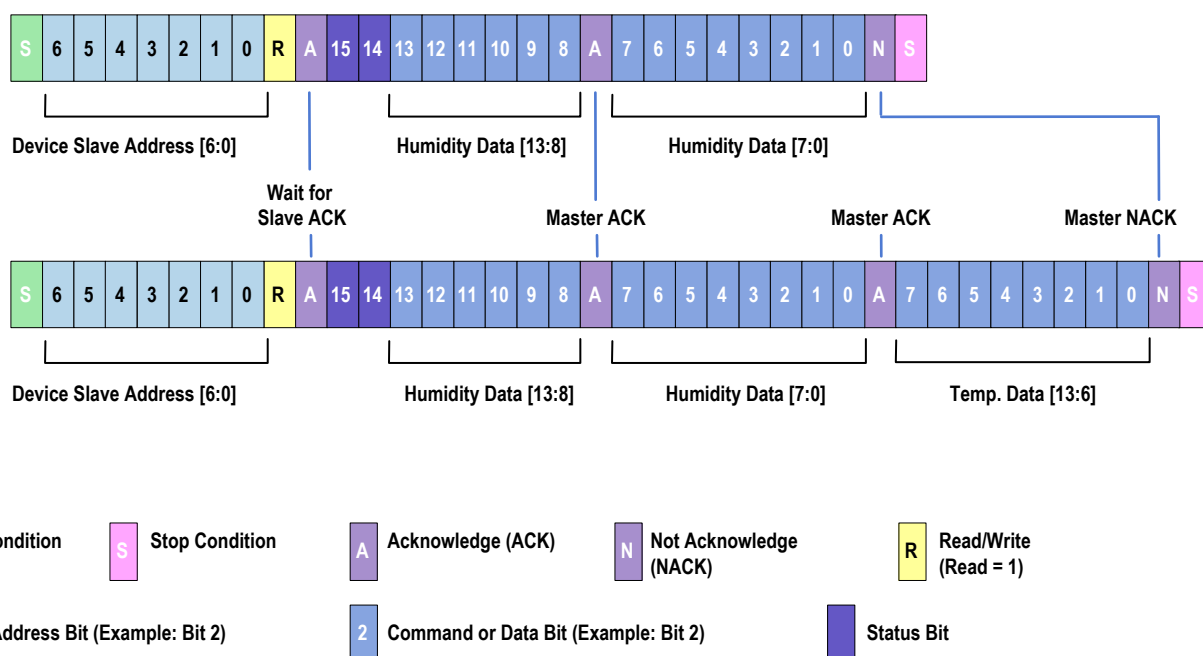
Figure 16. Data Fetch
