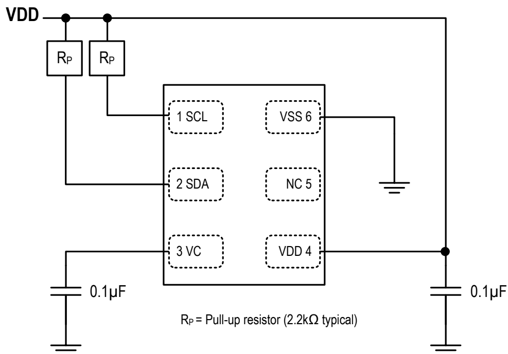
Figure 17. HS300x Application Circuit (Top View)
