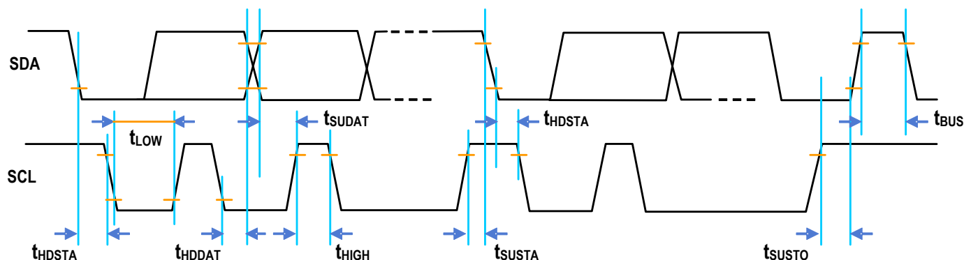
Figure 13. Timing Diagram
