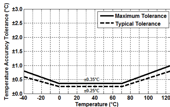
Figure 11. HS3003 Temperature Sensor Accuracy Tolerance
