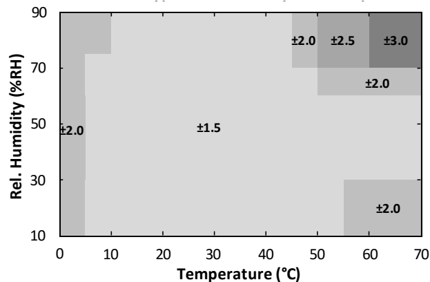
Figure 3. HS3001 RH Accuracy over Temperature
