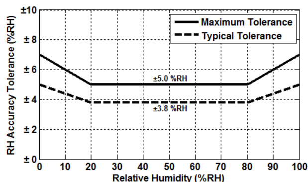
Figure 8. HS3004 RH Accuracy Tolerance at 25°C
