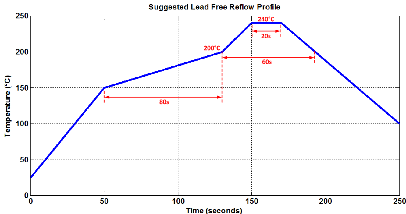
Figure 15. Recommended Soldering Profile
