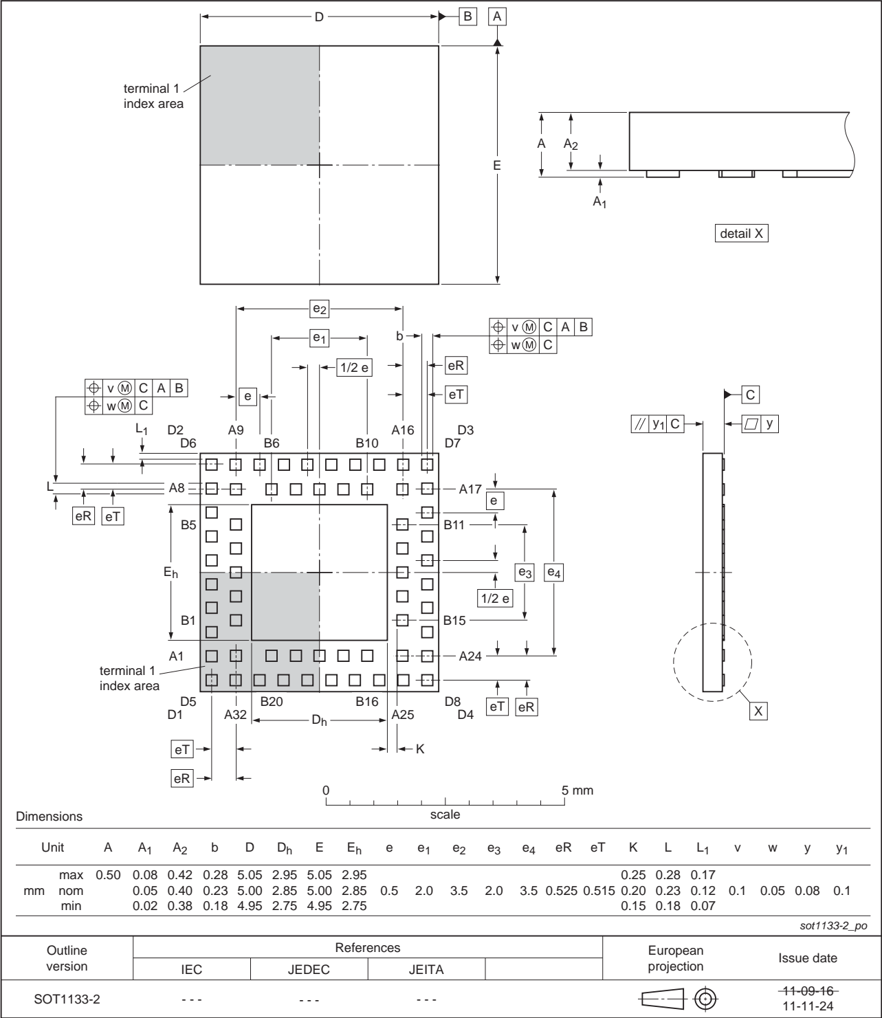
Fig 26. Package outline SOT1133-2 (HXQFN60)
