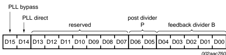
Fig 12. PLL register
