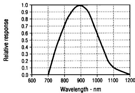
Fig. 3 Spectral Responsivity
