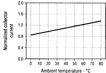
Fig. 2 Collector Current vs Ambient Temperature
