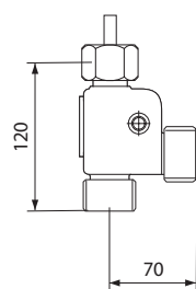
Comb. piece KF2
