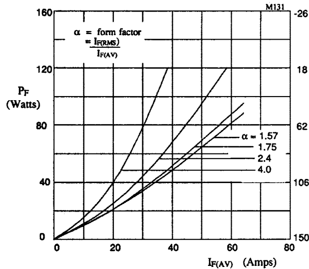
Figure 9. Forward power dissipation and maximum allowable mounting base temperature as a function of forward current for sinusoidal operation, for SET05**11.
