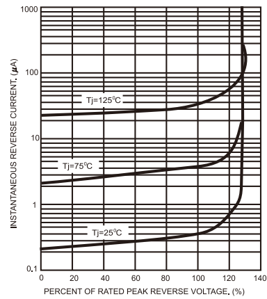
FIG.2- TYPICAL REVERSE CHARACTERISTICS
