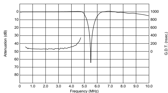
TPSKA5M50B00-R1
