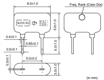
CDALF10M7C_Series
