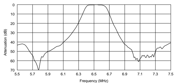
SFSKA6M50CF00-R1
