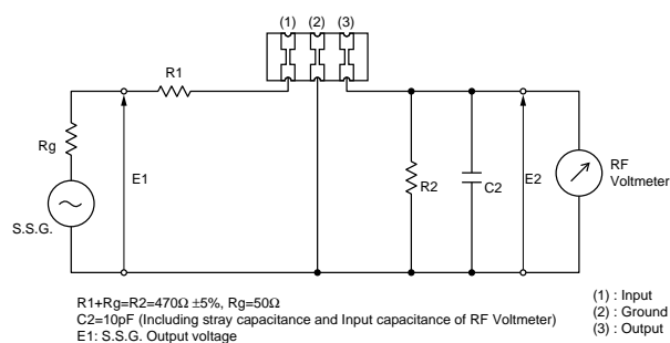
SFSKA6M50CF00-R1
