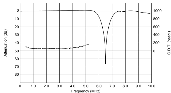
TPSKA6M50B00-R1
