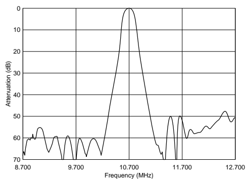
SFELF10M7HA00-B0
