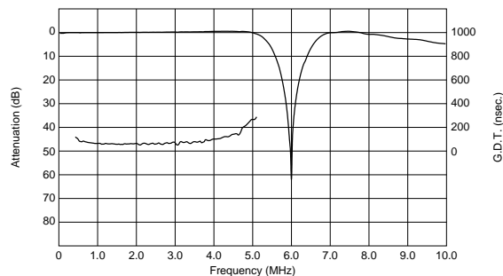
TPSKA6M00B00-R1
