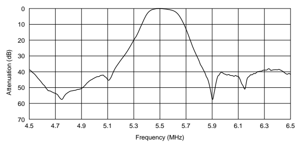
SFSKA5M50CF00-R1
