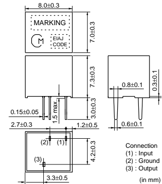
CFULA Series
