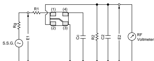
SFSKB2M80GF00-R1/SFSKB3M20FF00-R1
