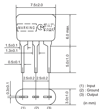
SFELG10M7HA00-B0
