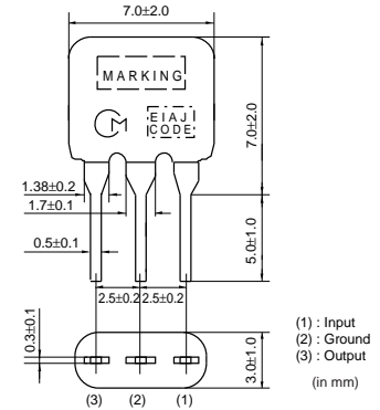
SFELF10M7HA00-B0
