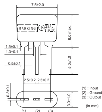
SFELG10M7KA00-B0
