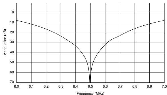
TPSKA6M50B00-R1
