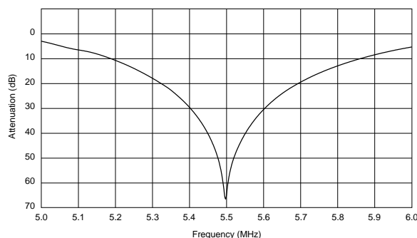
TPSKA5M50B00-R1
