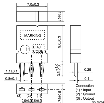
SFULA Series
