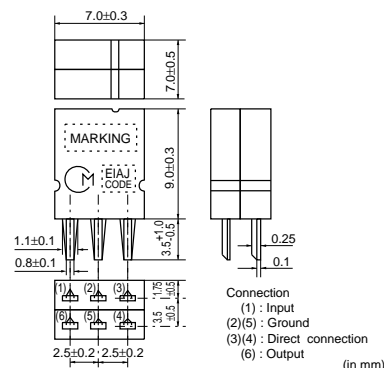
SFZLA Series
