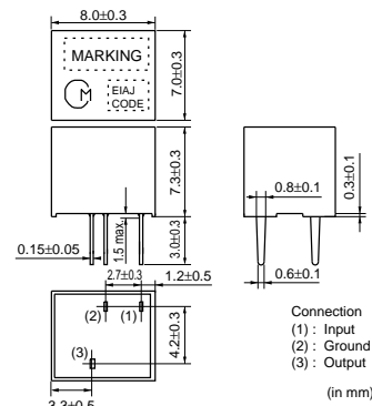
SFPLA Series
