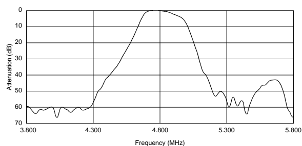
SFSKB4M80GF00-R1
