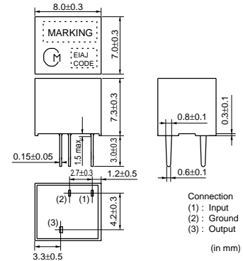
SFPLA Series
