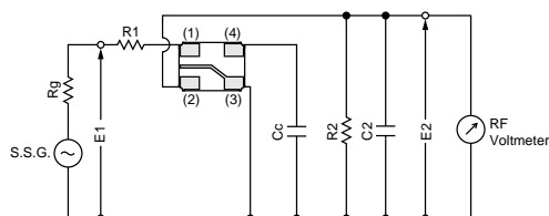
SFSKB5M20GF00-R1
