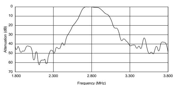
SFSKB2M80GF00-R1
