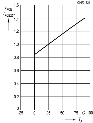
Photocurrent Fotostrom I_{PCE} / I_{PCE}(25^\circ\text{C}) = f(T_A), V_{CE} = 5\text{ V}
