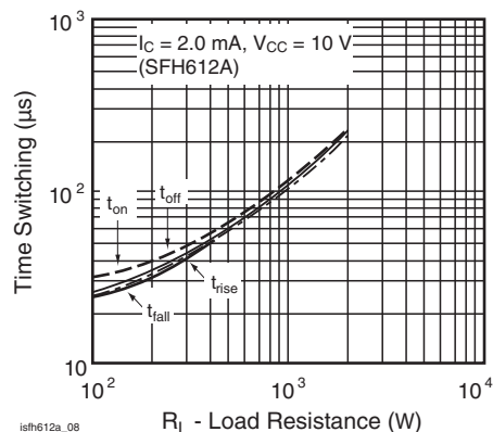
Fig. 11 - Switching Time vs. Load Resistor
