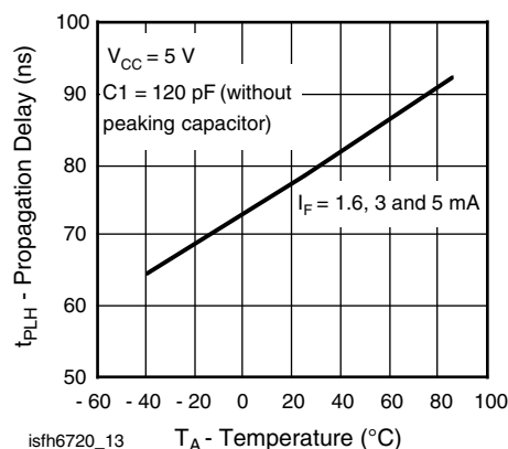
Fig. 13 - Typical Propagation Delays to Logic High vs. Temperature
