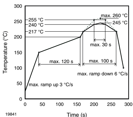
Fig. 25 - Lead (Pb)-Free Reflow Solder Profile According to J-STD-020 for SMD Devices
