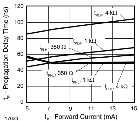
Fig. 18 - Propagation Delay vs. Forward Current
