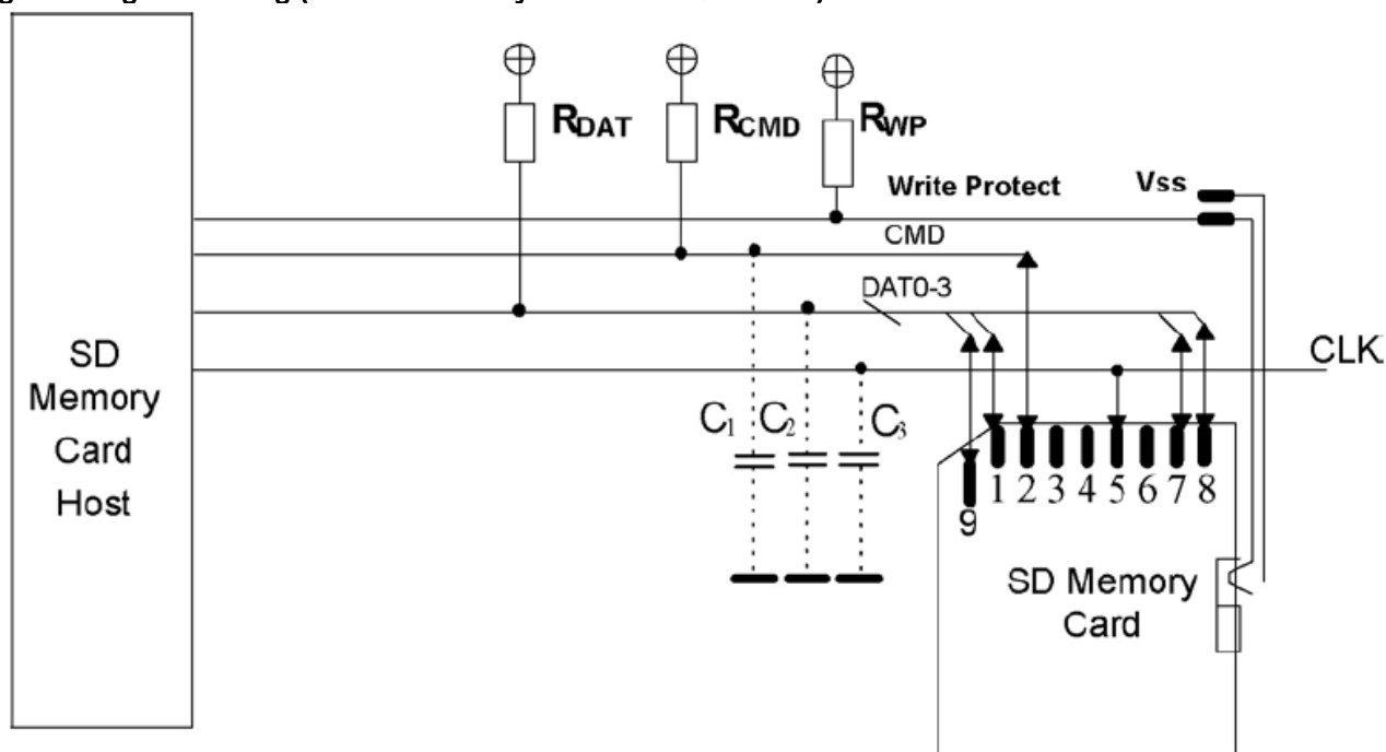
Figure 6: Signal Loading (Micro SD Memory Card has no WP slider)
