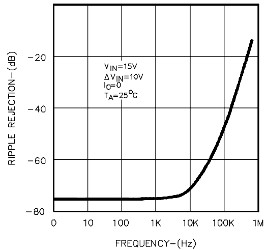
FIGURE 2. RIPPLE REJECTION
