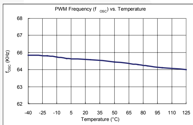
Figure 8. PWM Frequency
