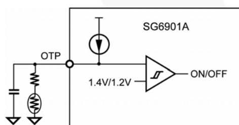
Figure 30. OTP Function
