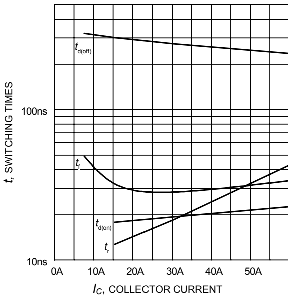
Figure 9. Typical switching times as a function of collector current (inductive load, T_J=150^\circ\text{C} , V_{CE}=400\text{V} , V_{GE}=0/15\text{V} , R_G=11\Omega , Dynamic test circuit in Figure E)
