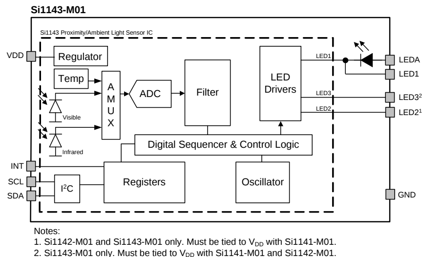
Figure 1. Si1143-M01 Sensor Module
