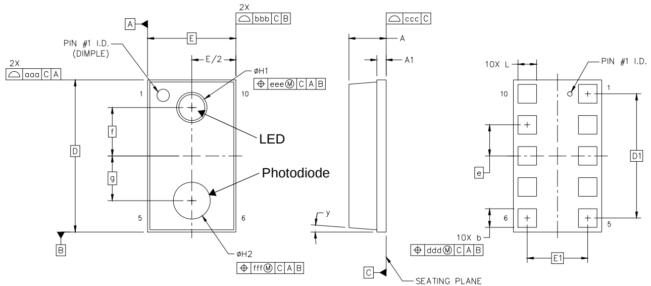
Figure 20. QFN Package Diagram Dimensions
