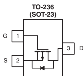
Top View Si2303CDS (N3)* * Marking Code
