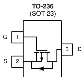
Top View Si2319DS (C9)* *Marking Code
