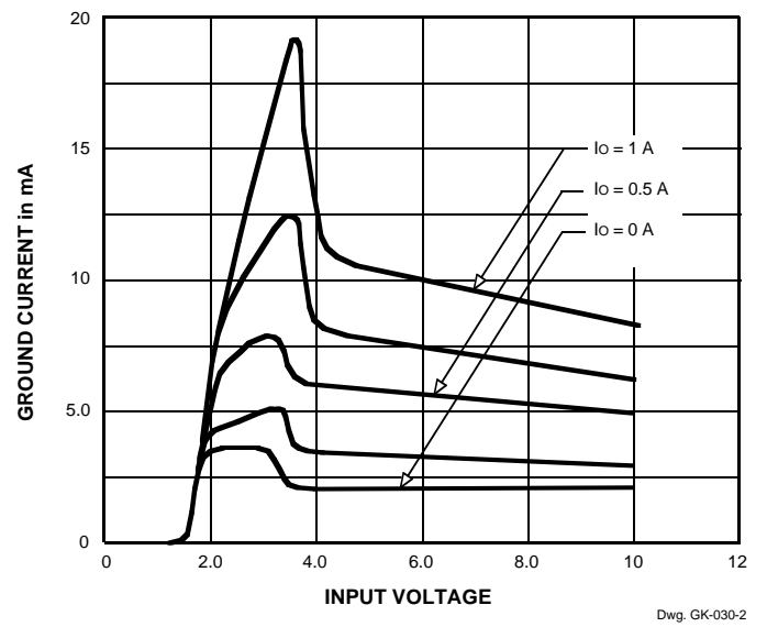
GND current
