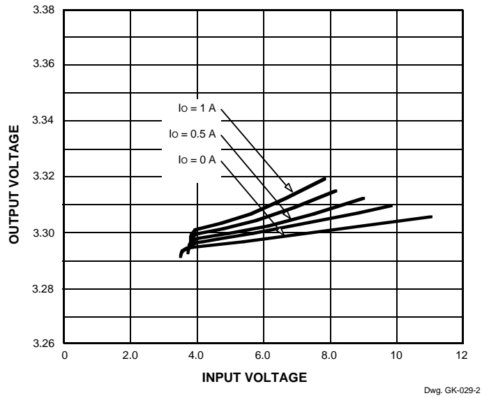
Line regulation
