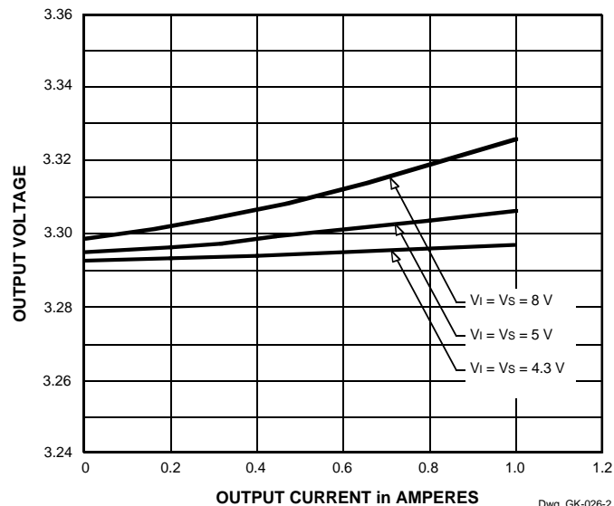
Load regulation
