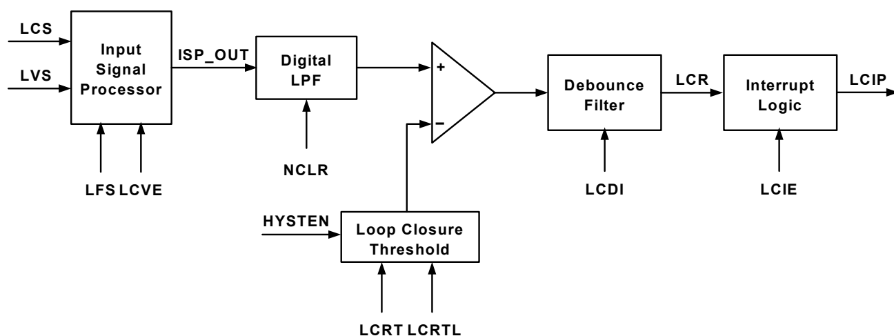
Figure 9. Loop Closure Detection
