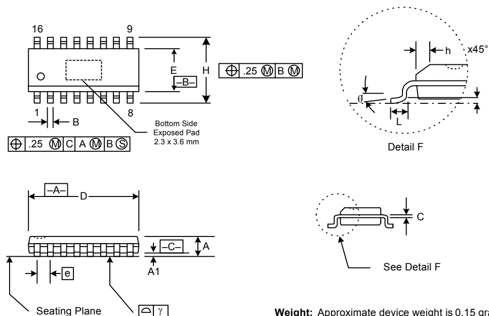
Figure 20. 16-pin Small Outline Integrated Circuit (SOIC) Package
